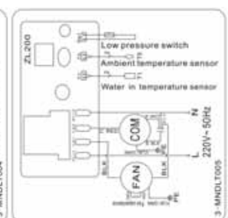
Heatermax COMPACT 20
