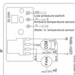
Heatermax COMPACT 10
