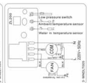
Heatermax COMPACT 20
