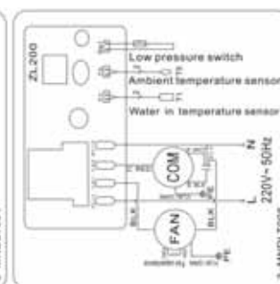
Heatermax COMPACT 20
