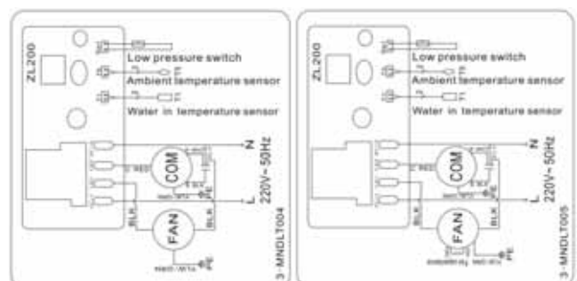
Heatermax COMPACT 10
